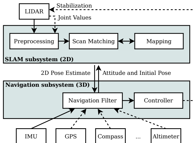
Fig. 1. Overview of the mapping and navigation system (dashed lines depict optional information)
